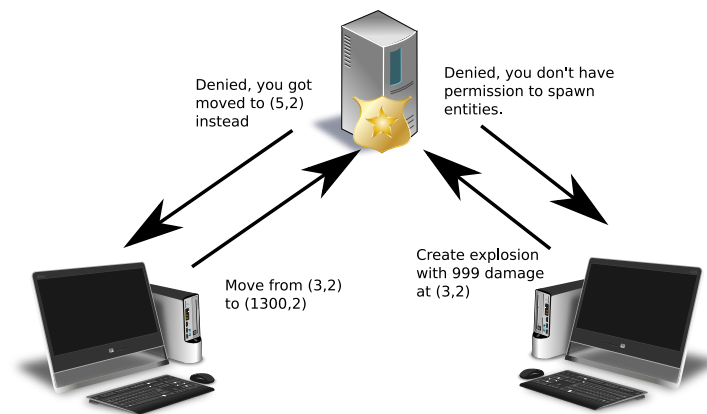
Figure 434: Two cheaters vs. Dedicated server
